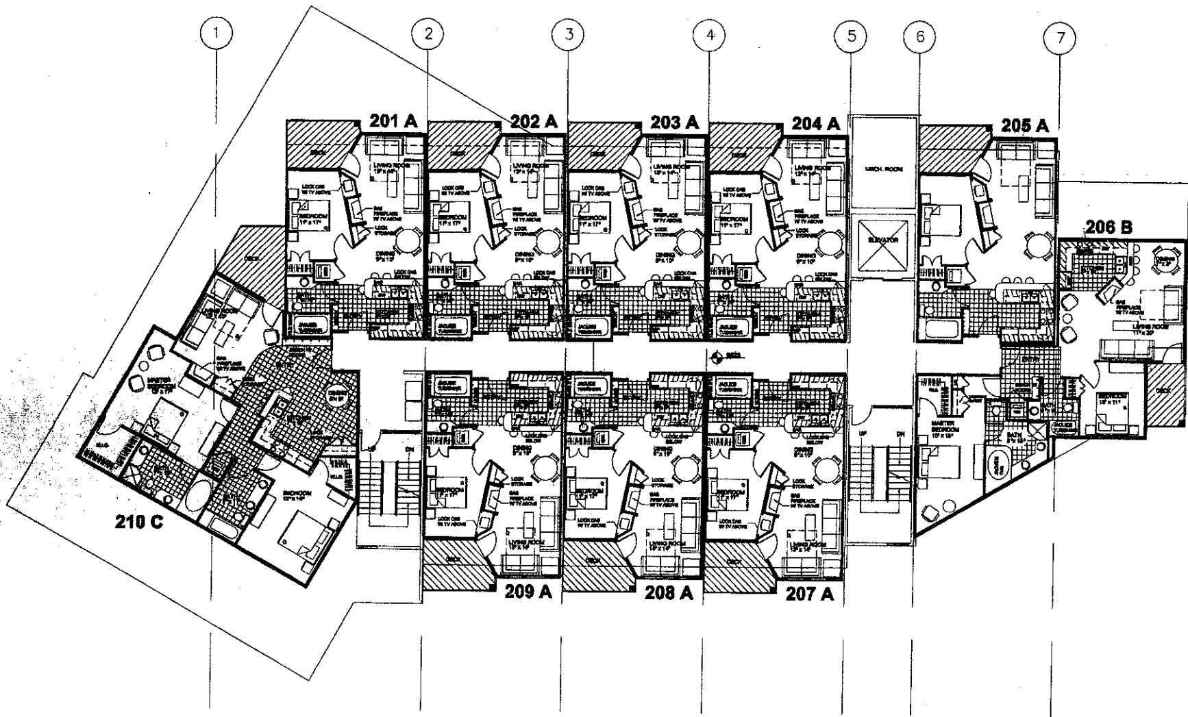
SECOND LEVEL FLOOR PLAN
