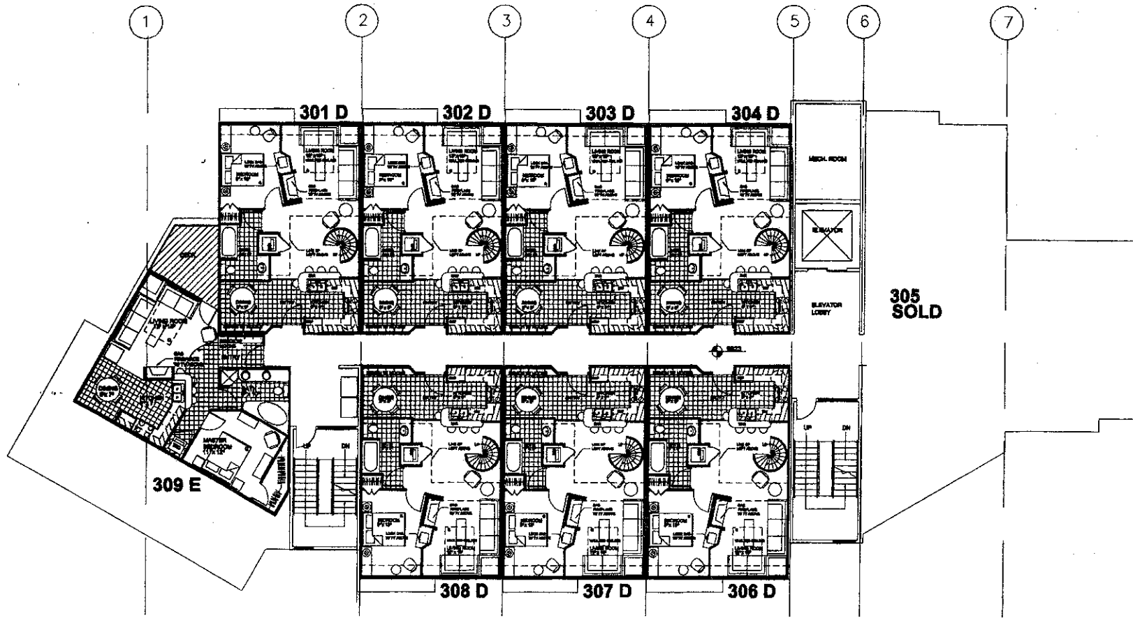
THIRD LEVEL FLOOR PLAN
