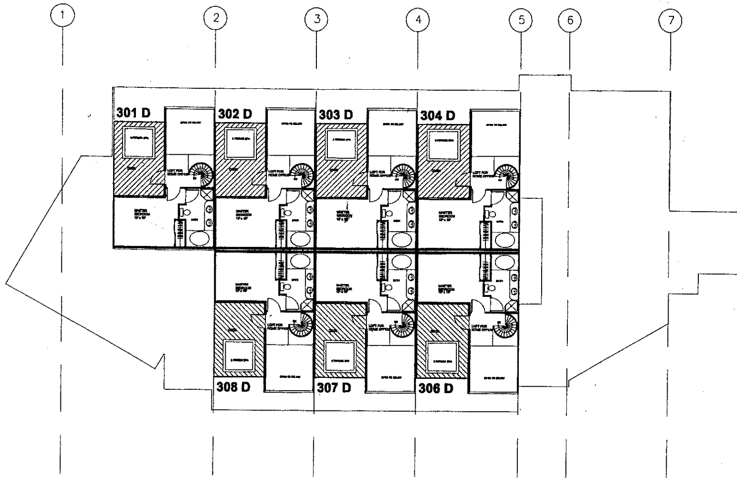
LOFT LEVEL FLOOR PLAN
